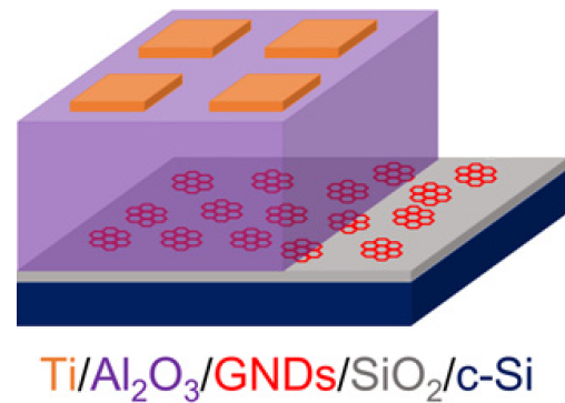
Fig. 1. Scheme of graphene nanodisk memory [16]
